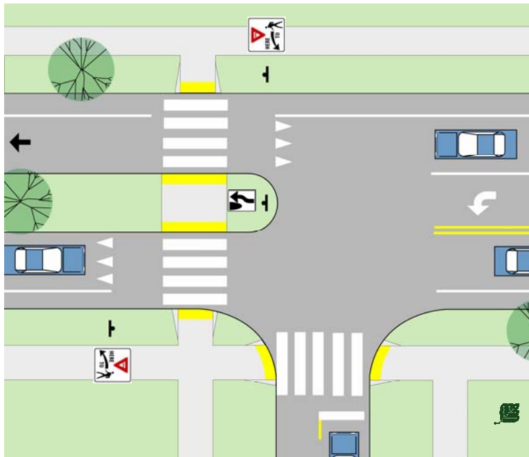
Fig. 2.4S. Unsignalized Tee Intersection with Turn Lane Guidelines
