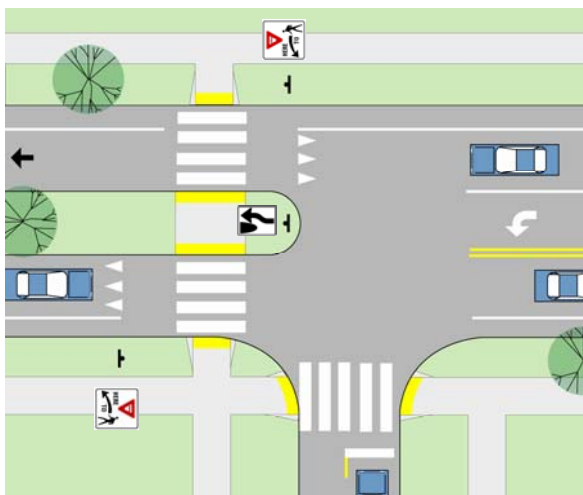
Figure 2.4A. Pedestrian Crossing island
