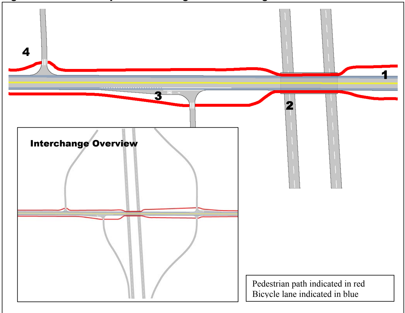
Fig. 2.4K. Urban Overpass Interchange Retro-fit Design Guidelines
