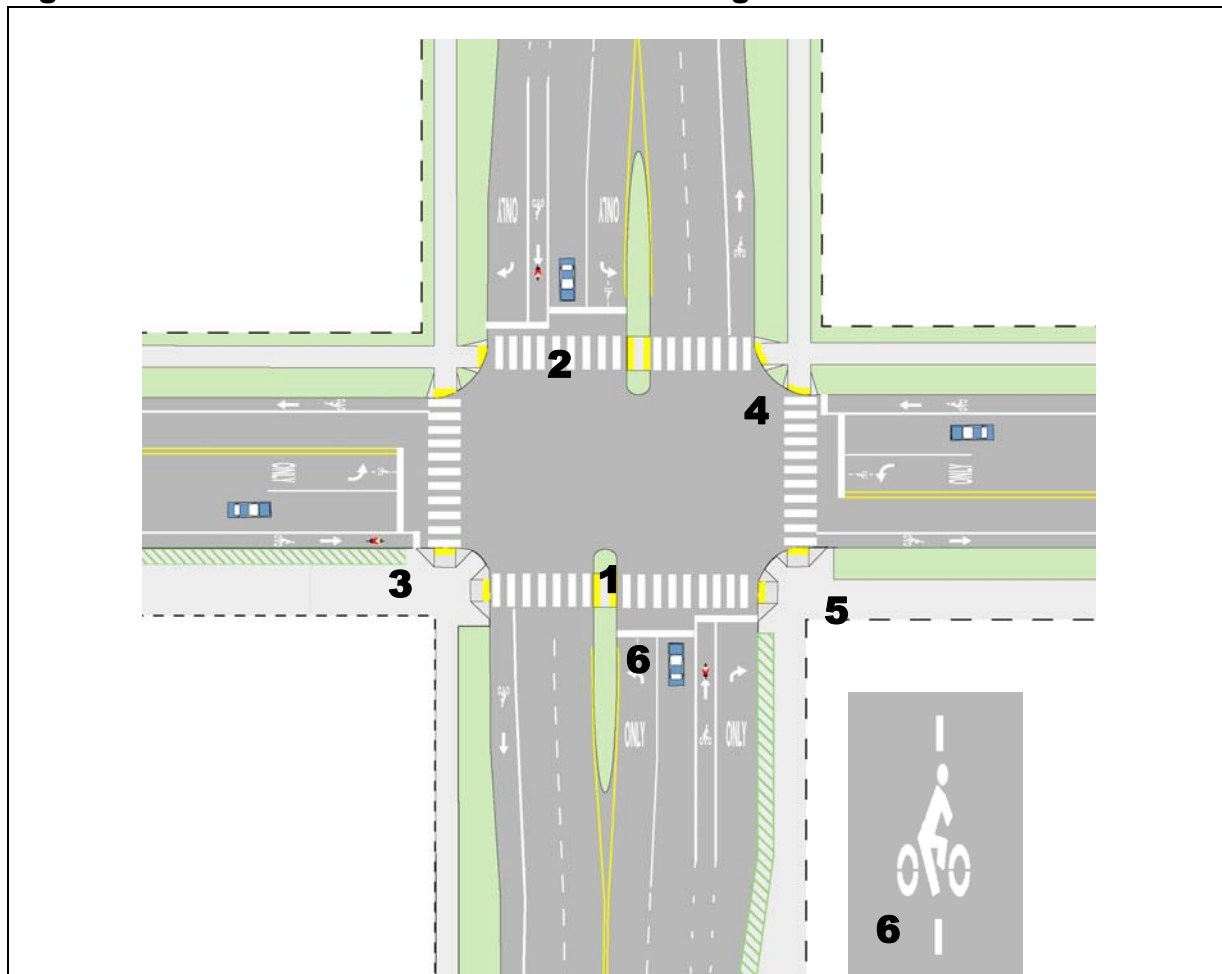
Fig. 2.4J. Multi-lane Urban Intersection Design Guidelines
