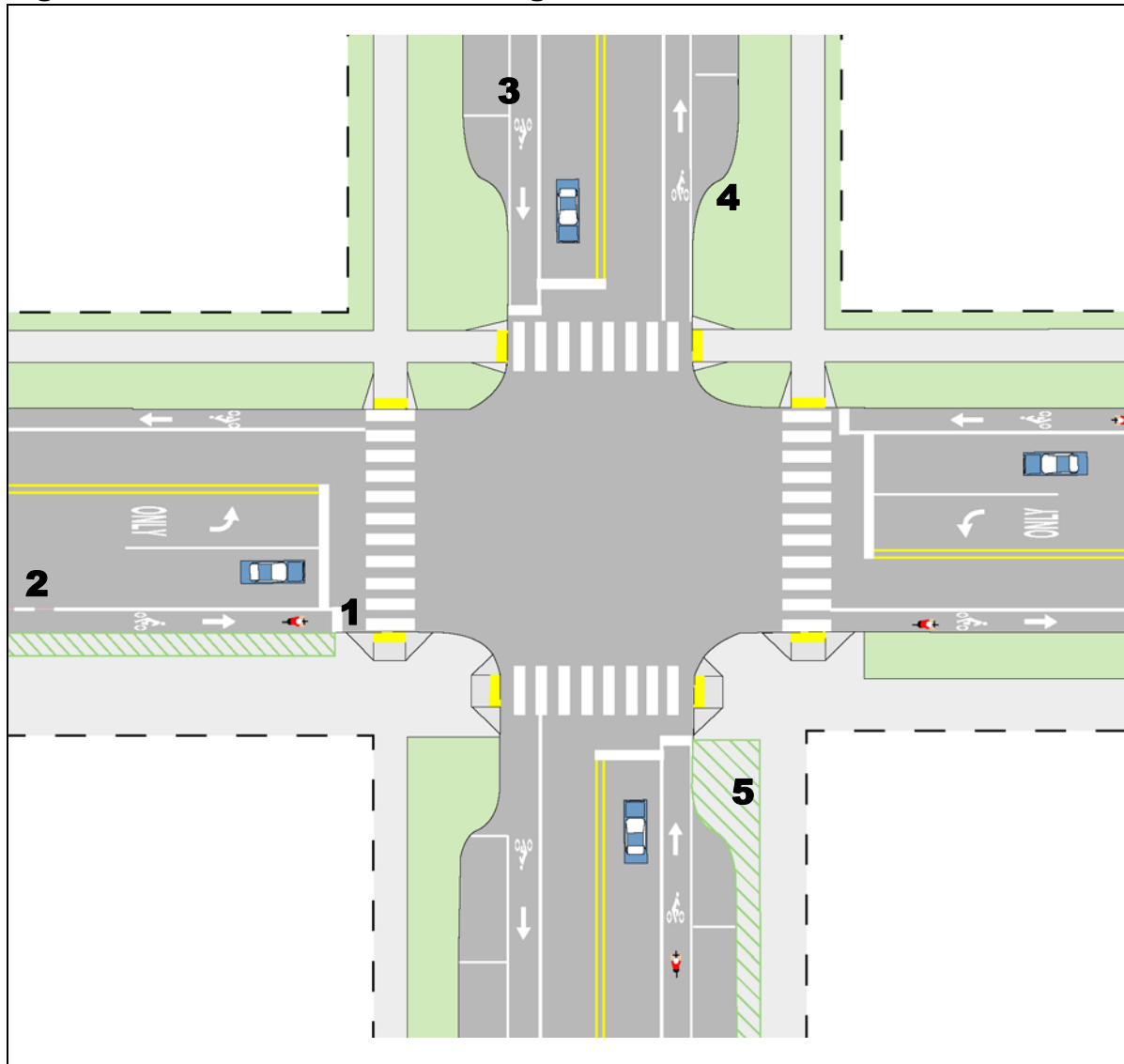
Fig. 2.4I. Urban Intersection Design Guidelines
