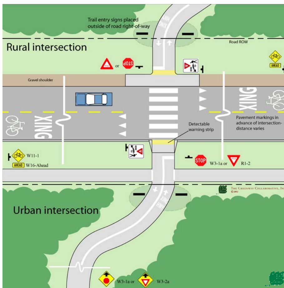
Fig. 2.5B. Typical Pathway/Roadway Intersection
