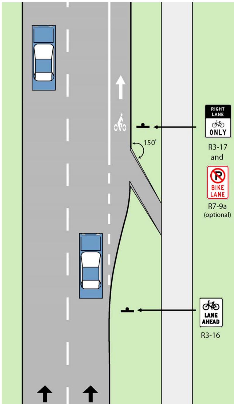
Fig. 2.3K. Bicycle Entrance Ramp from Sidewalk Bikeway to Bike Lane Design Guideline:
