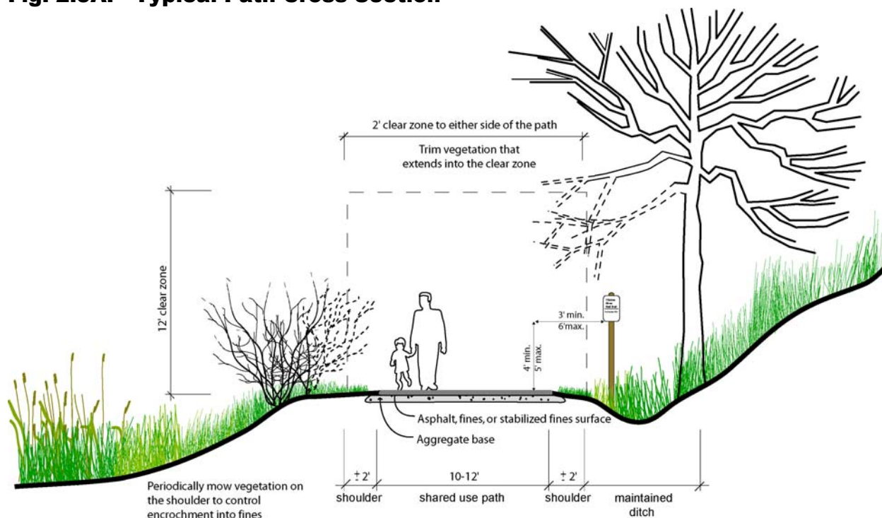
Fig. 2.5A. Typical Path Cross Section
