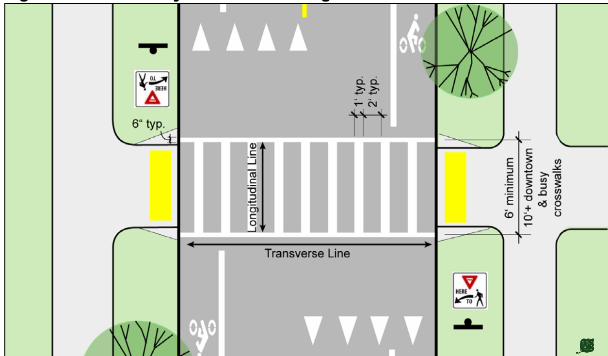
Fig. 2.4AB. Ladder Style Crosswalk Design Guidelines
