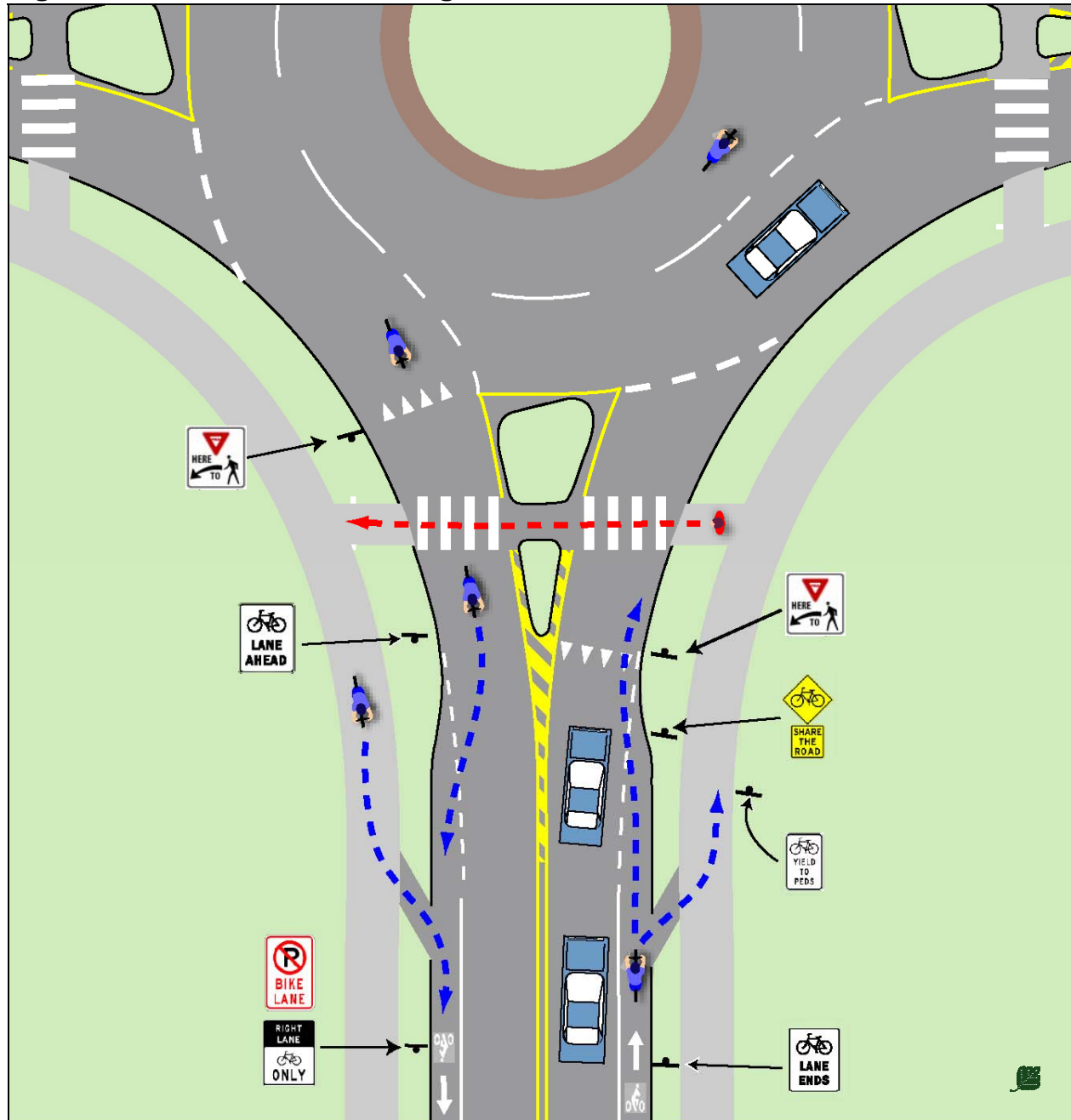
Fig. 2.4AA. Non-motorized Design Considerations for Roundabouts
