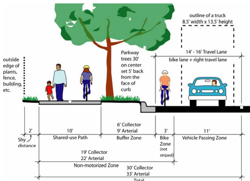
Fig. 2.3D. Scenario C – Shared-use Path
