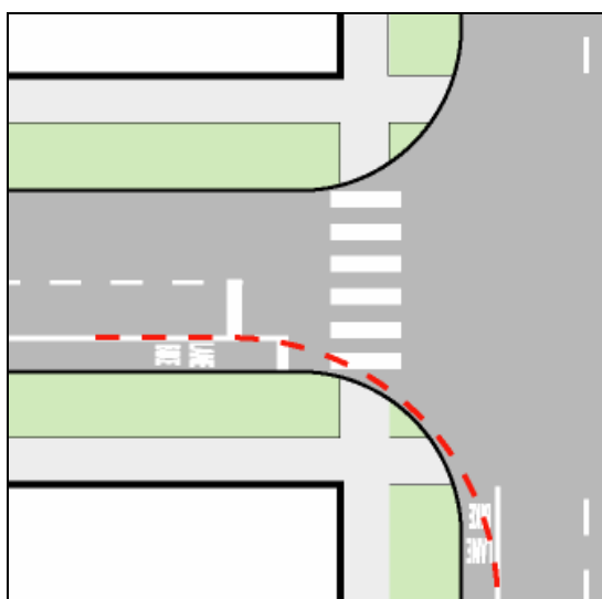
Fig 2.4C. Effect of Bike Lanes on Turning Radius
